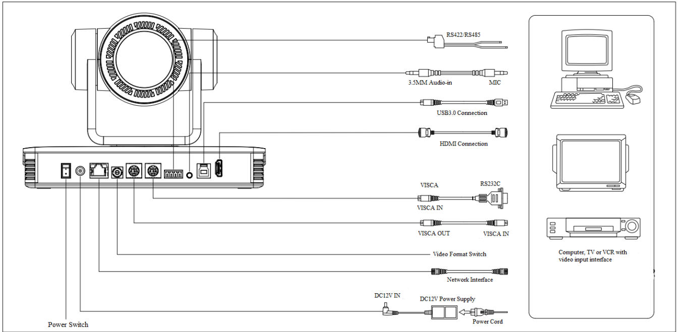
Figure 2.5 Wiring Diagram
